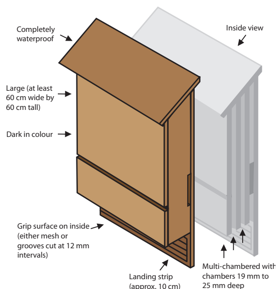
KEY FEATURES OF A BAT-HOUSE DEMONSTRATED WITH FOUR-CHAMBER NURSERY HOUSE
